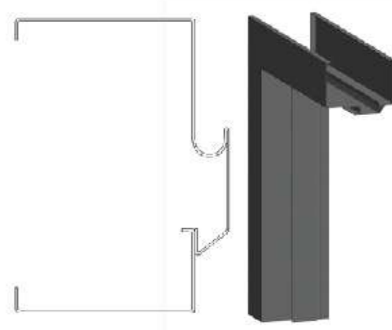
Adjustable Frame Type II
